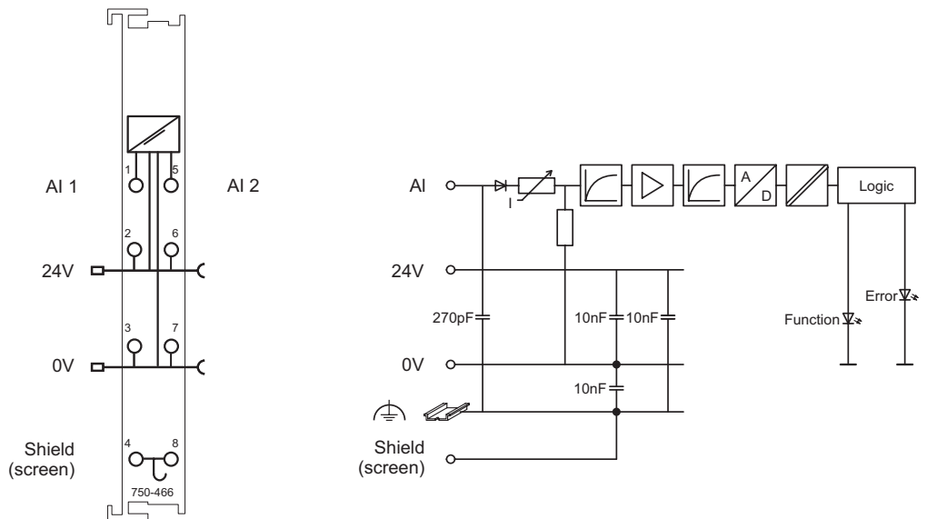
Fig. 2.1.1-3: Schematic Diagram
